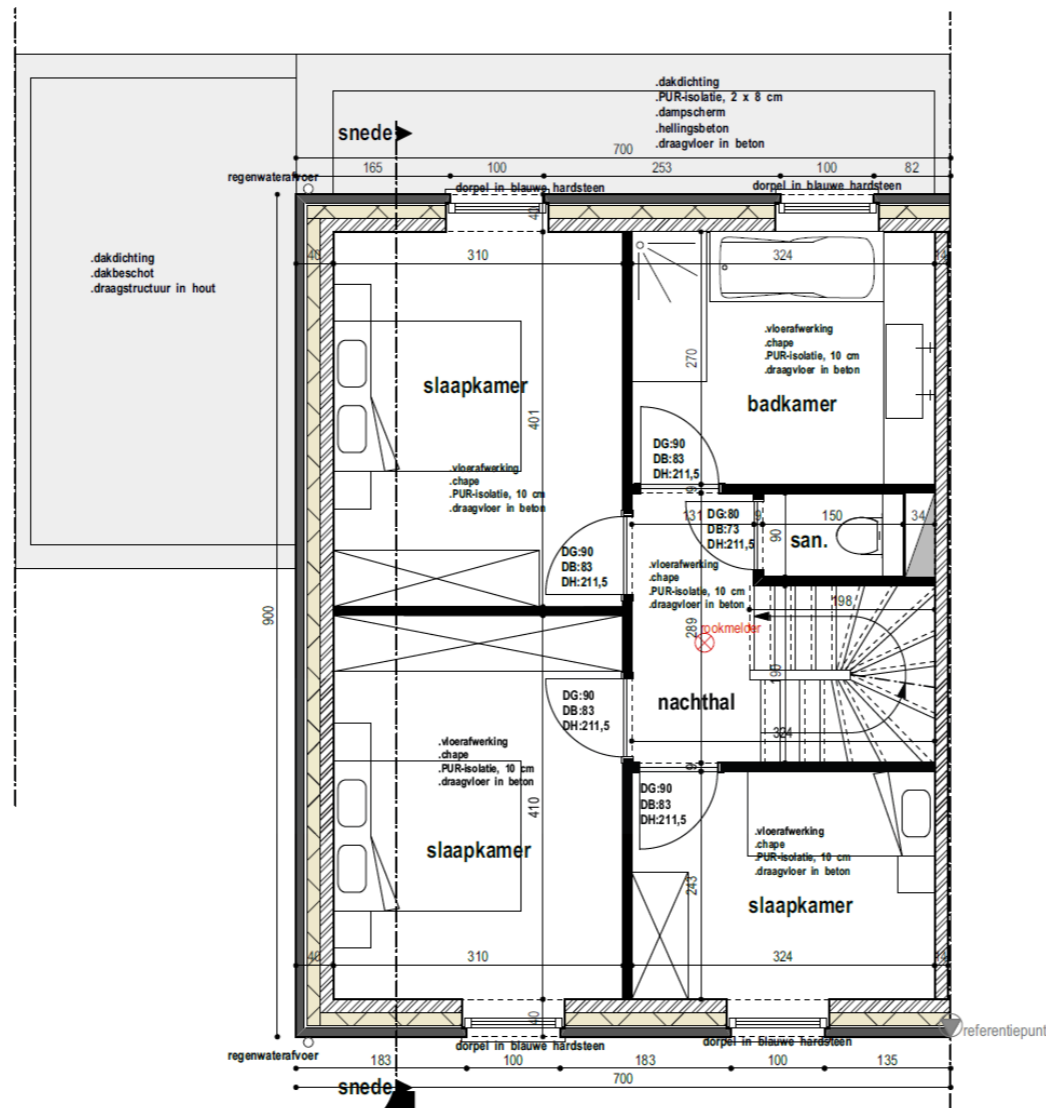
+1 schaal 1:50
